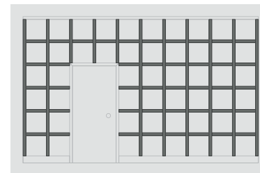
FIELD STILES & RAILS: 1 1/2" X 1/4"
